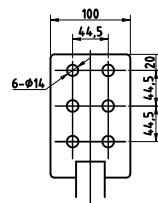
Lv bushing
